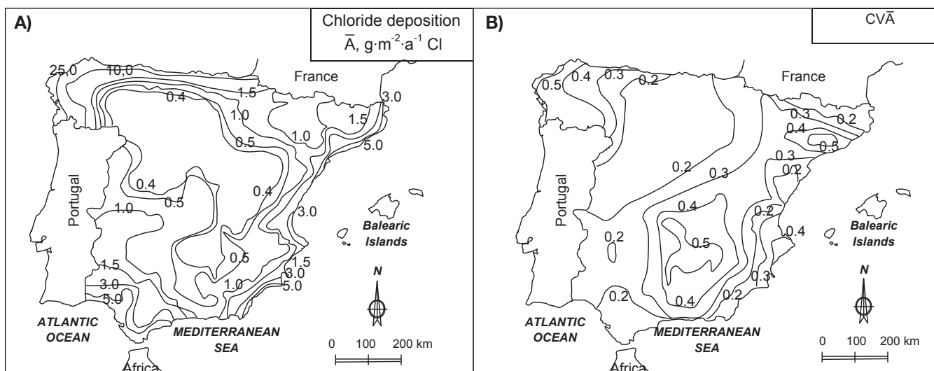
Fig. 5. Preliminary estimation of average atmospheric chloride deposition in conterminous Spain from 10 km × 10 km pixels, as calculated by Alcalá [1]. Contour lines are an approximation, modified from [1,15]. (A) Atmospheric deposition ( \text{g Cl m}^{-2} \text{ year}^{-1} ). (B) The coefficient of variation (standard deviation/mean), expressed as a fraction.
