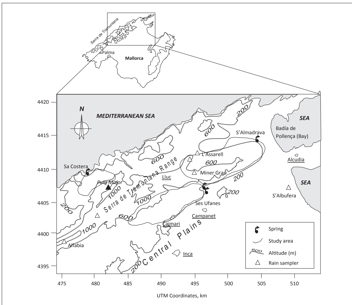
Fig. 4. The eastern Serra de Tramuntana range in the northern part of Mallorca. The bounded recharge areas correspond to the three main outflow springs: Sa Costera, the intermittently large spring Ses Ufanes, and S'Almadrava. Ses Ufanes is an overflow spring of the upper catchment area, with the remaining flow contributing to the S'Almadrava area.
