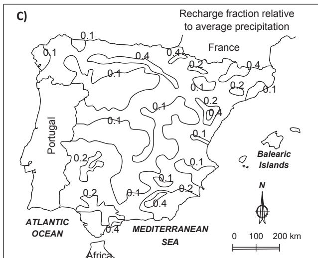
Fig. 9. Preliminary estimation of the fraction of precipitation that is virtual recharge in conterminous Spain, deduced from 10 \text{ km} \times 10 \text{ km} pixels, as calculated by Alcalá [1].
