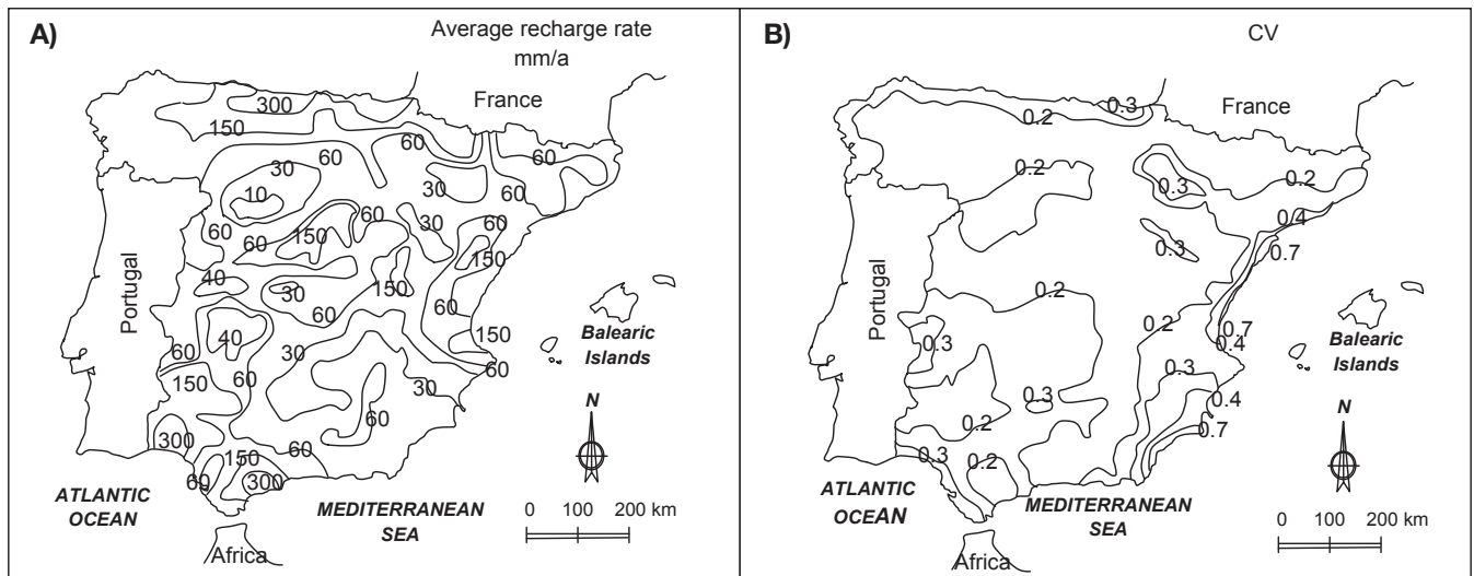
Fig. 8. Preliminary estimation of virtual average recharge rate in conterminous Spain, deduced from 10 \text{ km} \times 10 \text{ km} pixels, as calculated by Alcalá [1]. (A) Contour lines are an approximation of average recharge rates (mm/year), modified from [1,4]. (B) The coefficient of variation.
