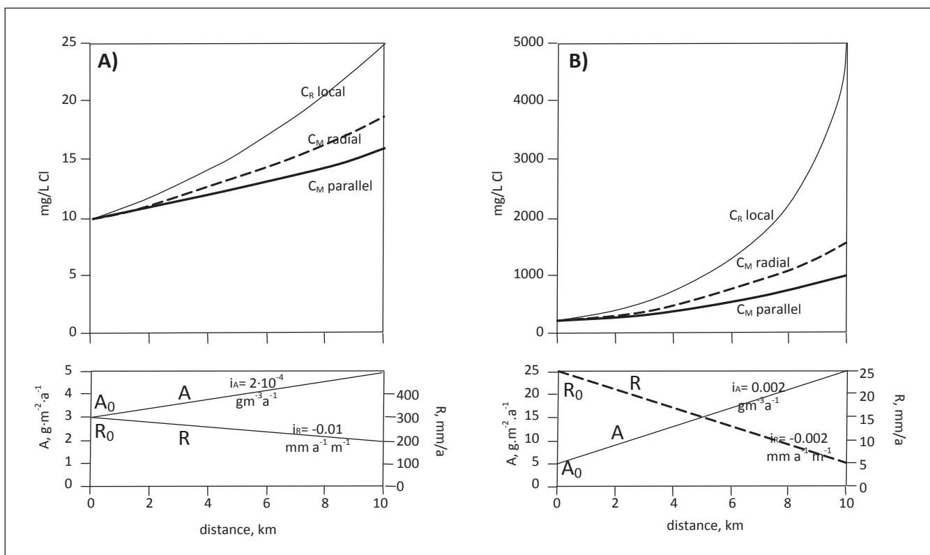
Fig. 2. Recharge in a sloping aquifer, showing chloride concentration in local recharge and the average value through the aquifer thickness, at increasing distance from the upslope boundary or apex in parallel flow and radial flow, respectively. (A) Well-recharged aquifer (humid climate) with slightly changing, moderate chloride deposition. (B) Poorly recharged aquifer (arid climate) with changing chloride deposition (proximity to the coast).
