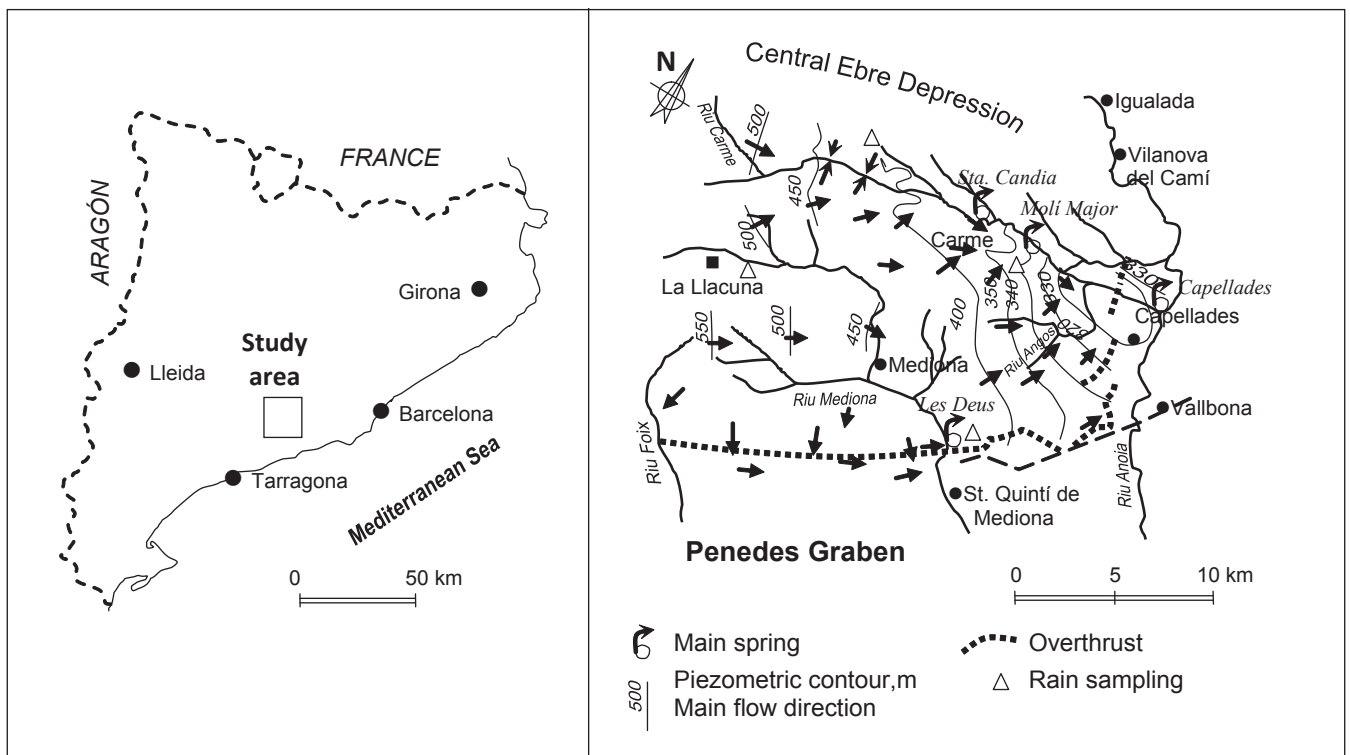
Fig. 3. The Anoia carbonate aquifer system (pre-littoral Catalan range, Barcelona) and the main discharge points (springs and the base flow of the Riera de Carme). The arrows indicate groundwater flow in the main recharge area [14,32].
