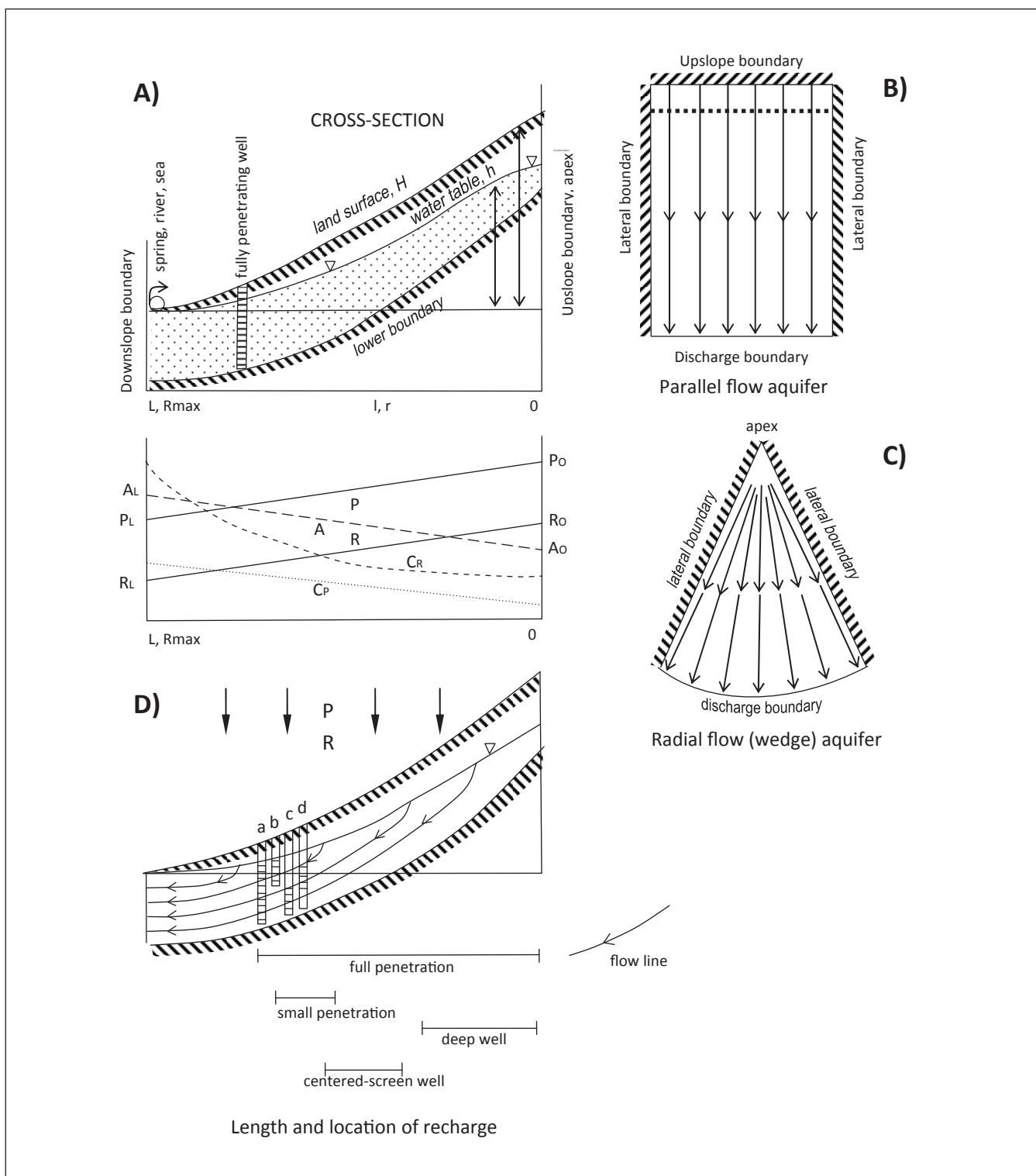
Fig. 1. Recharge in a sloping aquifer. (A) Cross-section and P (precipitation), R (recharge), A (atmospheric chloride deposition), C_p (chloride concentration in rainfall), and C_R (chloride concentration in recharge): qualitative variation along the flow. (B) Parallel flow aquifer. (C) Radial-flow aquifer. (D) Length and location of areal recharge mixing in wells according to the screen length and position, assuming the well does not significantly disturb of the groundwater flow pattern.
